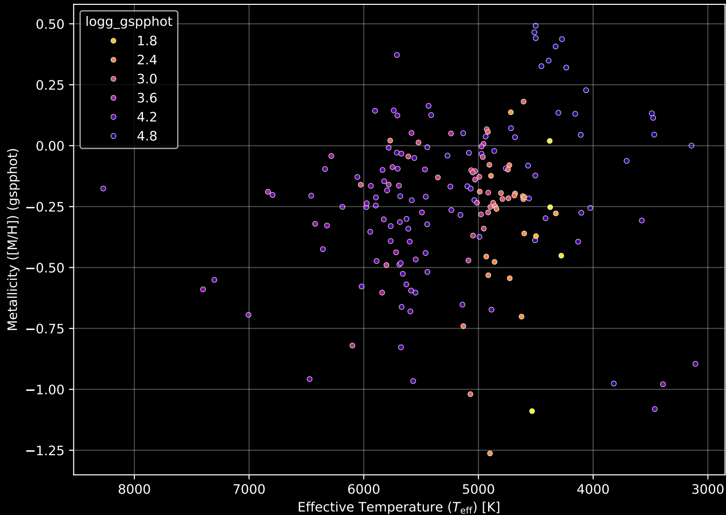
APOGEE DR17 Field: [058+39_MGA] Stellar Population Parameters (n= 177)
