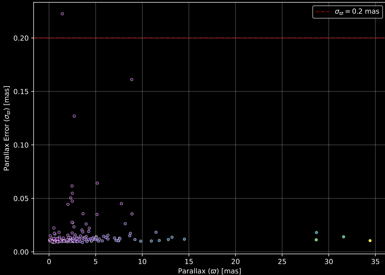
APOGEE DR17 Field: [058+39_MGA] Parallax Quality (n= 177)
