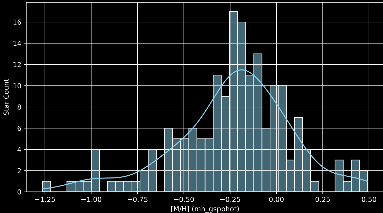
APOGEE DR17 Field: [058+39_MGA [M/H] (mh_gspphot) (n= 177)
