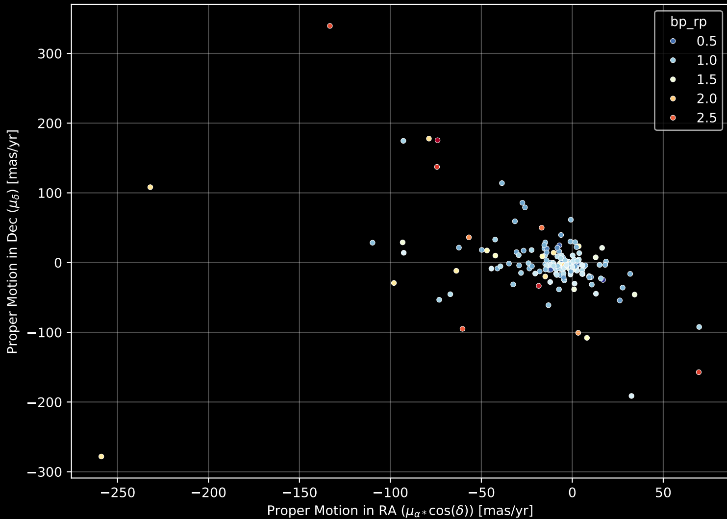
APOGEE DR17 Field: [058+39_MGA] Proper Motion Diagram (n= 177)
