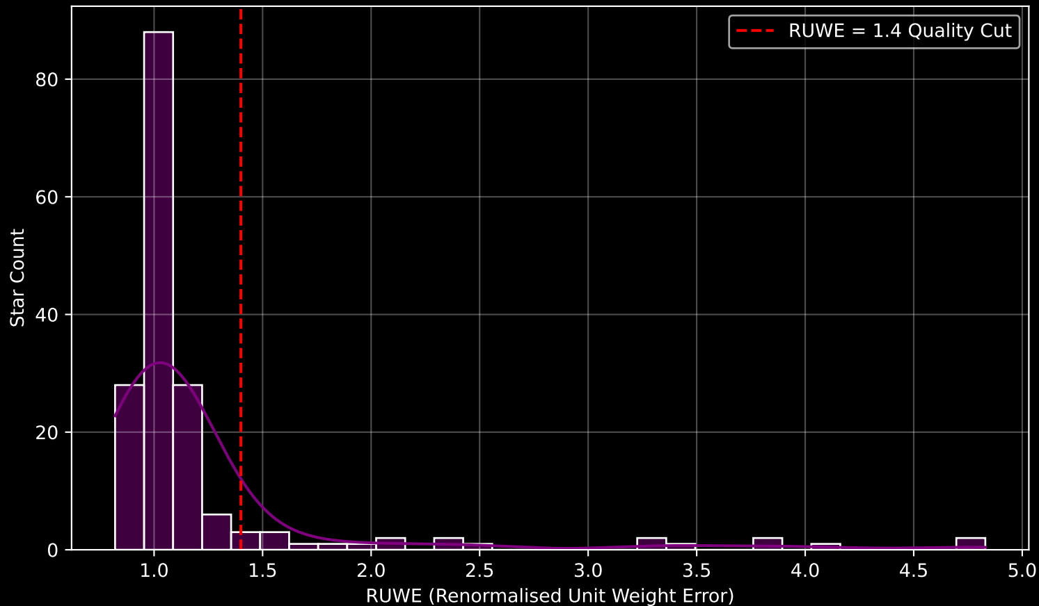
GAPOGEE DR17 Field [058+39_MGA] RUWE Distribution (n= 172)
